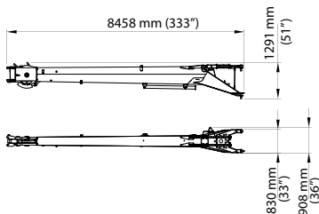
Fly jib - 8 m (26.3 ft)
